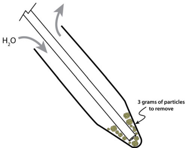
Fig. 3 “Fragment-clearance” system for testing the lithotrite, hands-free, with the probe angled downward. Time was measured for complete removal of ~2 mm test pellets
