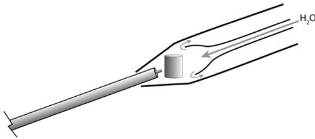
Fig. 2 “Movable-stone” system for testing lithotrite, hands-free, with the probe angled up, and the test stone resting in contact with the probe by gravity. A plastic funnel-tipped tube directed water toward the probe tip and confined the space occupied by stone fragments to ~3 ml. Time was measured for the lithotrite to break up the test stone and aspirate all fragments
