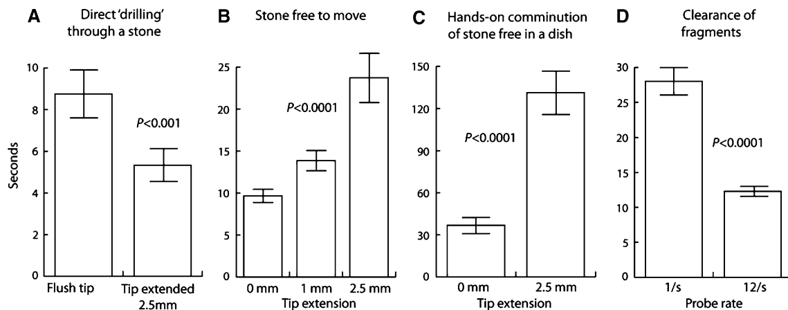
Fig. 4 Effect of ballistic probe settings on lithotrite performance in vitro. Time needed to drill through a stone held in fixed position (as in Fig. 1) was faster when the inner probe was extended (a), but having the tip project beyond the outer probe reduced the efficiency of com-
